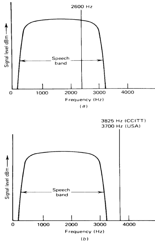
Fig. 2.2 SF signaling (a) in-band and (b) out-of-band.
