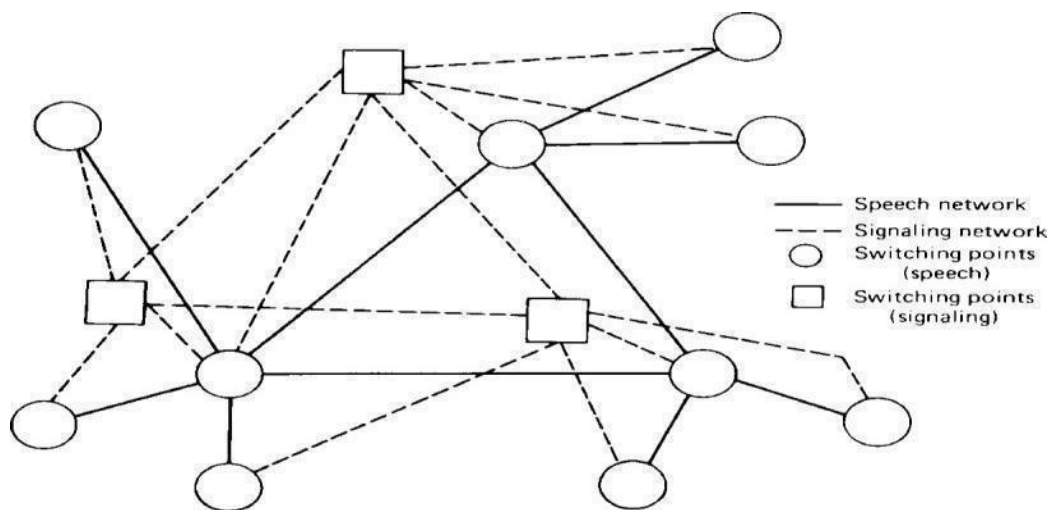
Figure 2.7 Fully disassociated channel signaling. This signaling may be used with CCITT Signaling System No. 7.
