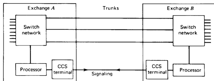
Separate Channel Signaling
