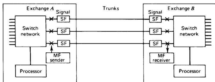
Associated Channel Signaling (Conventional SF-MF)
