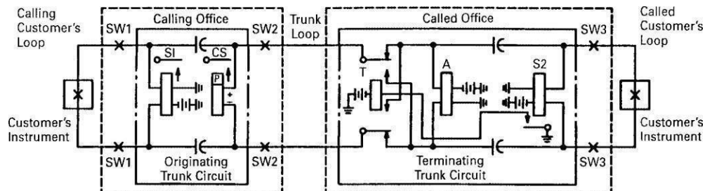
Figure 2.10 Reverse-battery signaling
