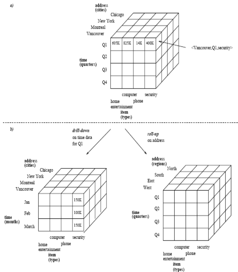
A multidimensional data cube, commonly used for data warehousing, a) showing summarized data for and b) showing summarized data resulting from drill-down and roll-up operations on the cube in a .
