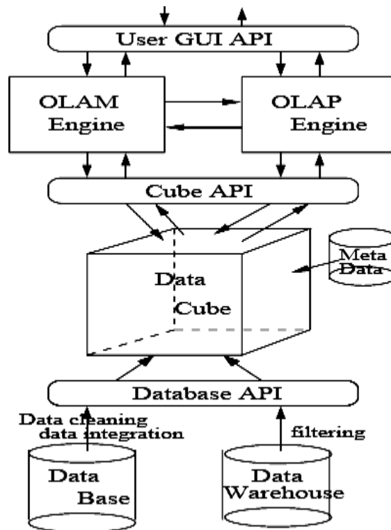
Figure: An integrated OLAM and OLAP architecture.
