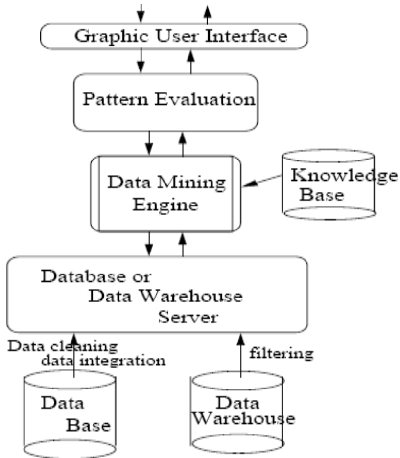
Architecture of a typical data mining system.
