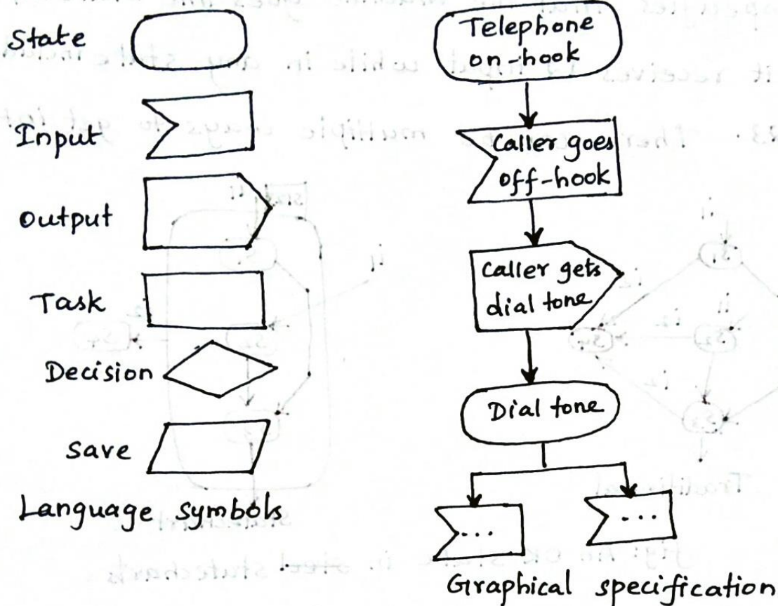
fig: The SDL Specification language
