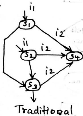
fig: An OR state in statecharts.
