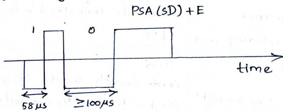
Bit encoding in DCC
