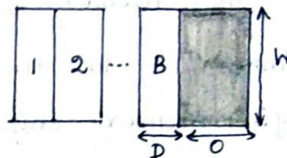
fig: Times & data volumes in a burst bus transfer
