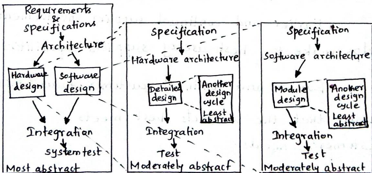
fig: A hierarchical design flow for an embedded system
