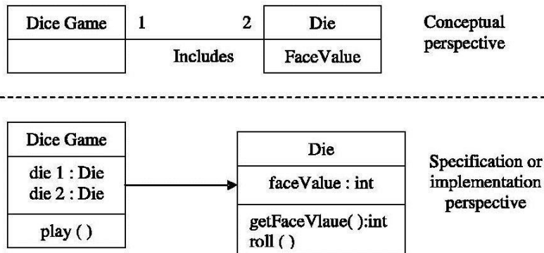
Figure 1.8 Different Perspectives with UML
