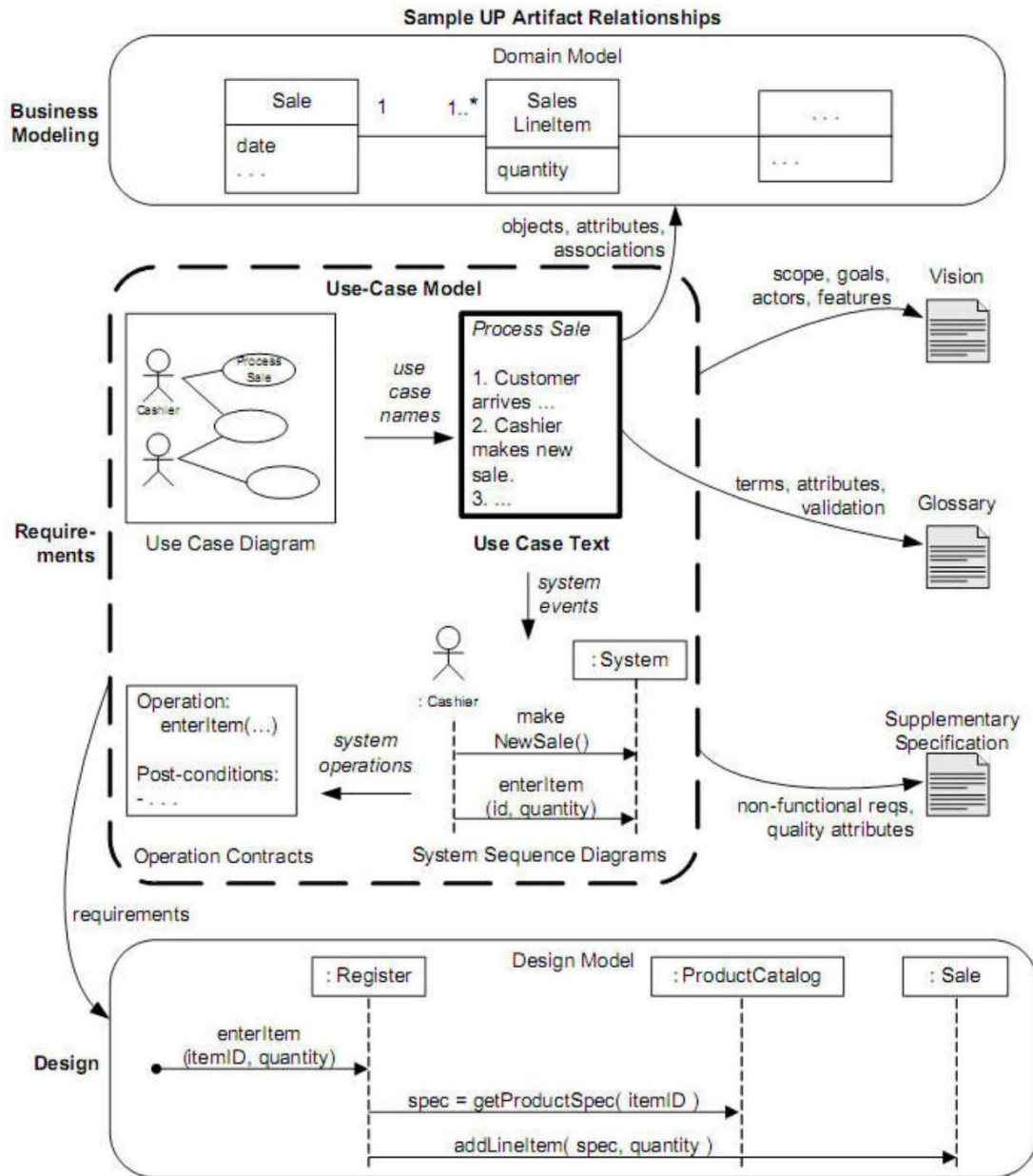
Figure 1.13 Sample UP Artifacts Relationships
