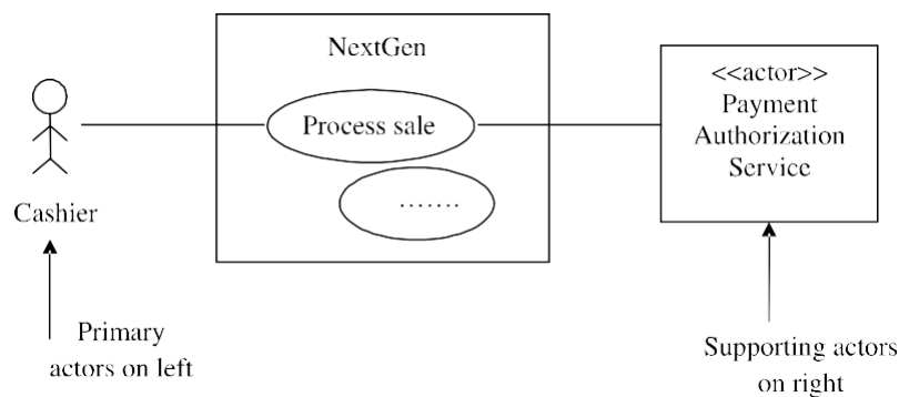
Figure 1.15 a) Notation of actor
