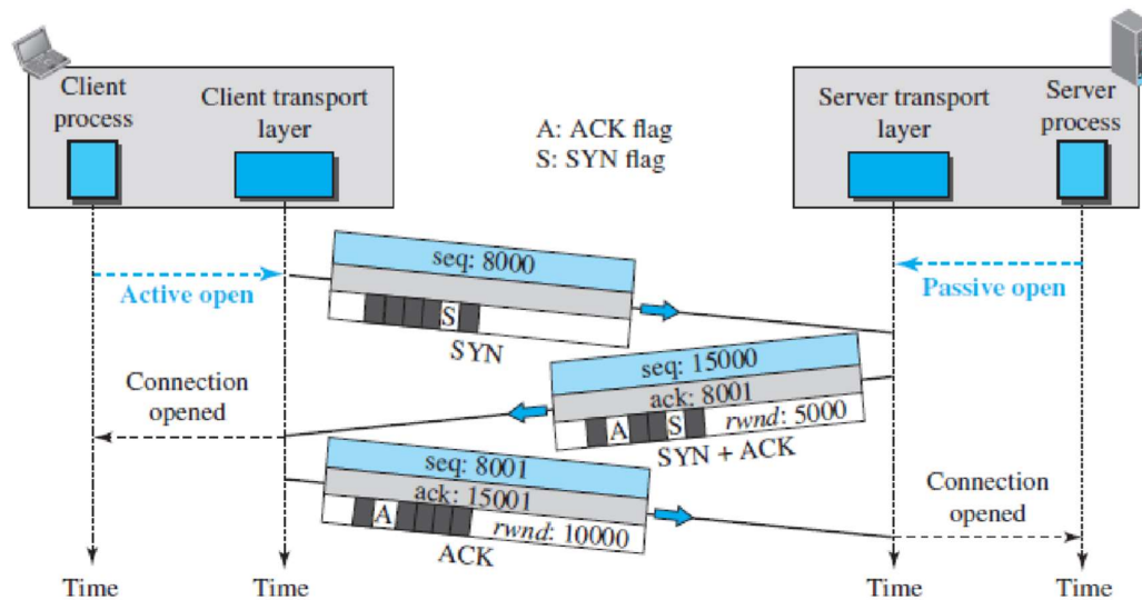
Fig4.3.1:TCP connection.
