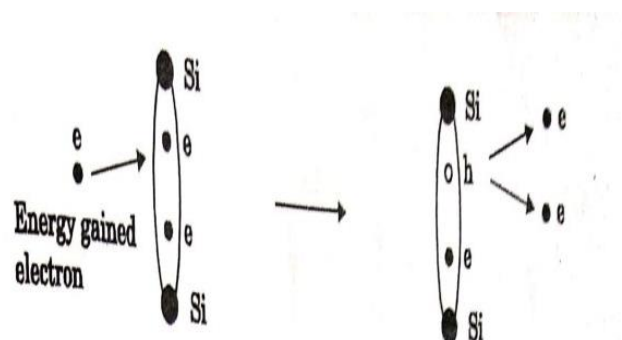
Fig 4.2.3. Impact Ionization
