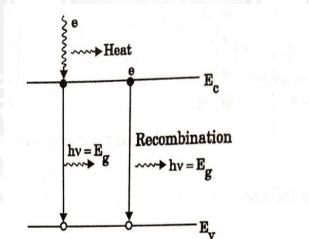
Fig 4.2.4. Radiative Recombination
