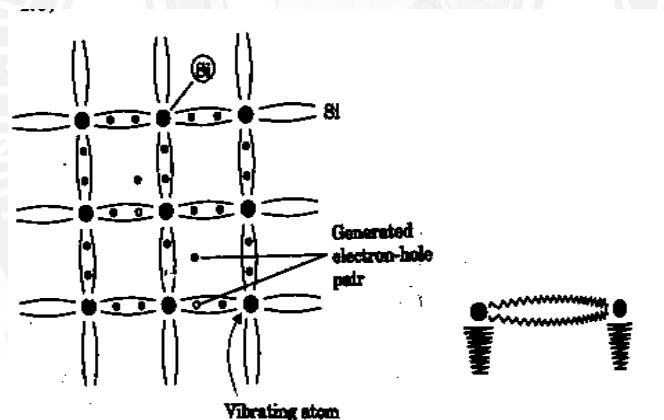
Fig 4.2.2 Phonon Regeneration
