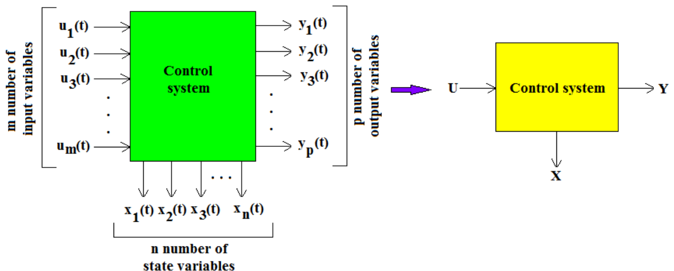
Figure 5.1.1 State space representation of a system
