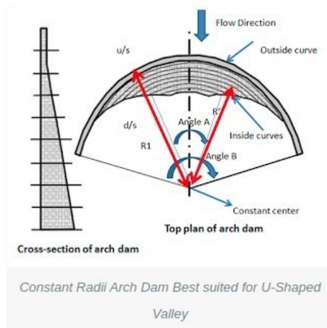
Constant Radii Arch Dam Best suited for U-Shaped Valley
