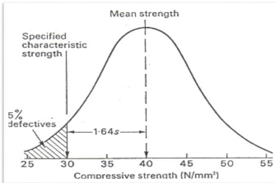
Compressive strength (vs.) Characteristic compressive strength
