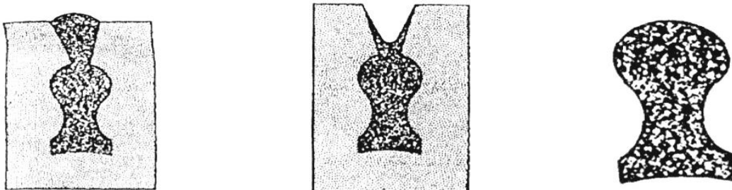
Fig. 4.5.1- Solid slip casting
