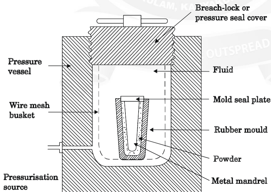
Fig. 4.5.2: Wet-bag isostatic pressing system
