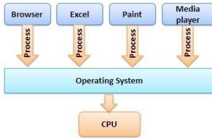
Figure: Multitasking
