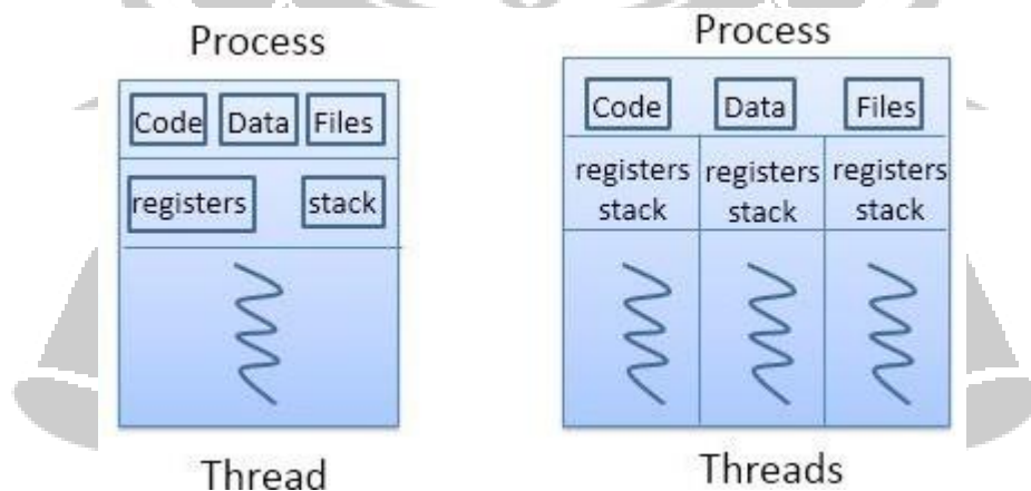
Figure: Multithreading
