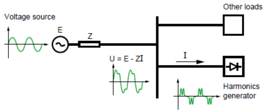
Figure 5.5.1 Degradation of network voltage due to non-linear load
