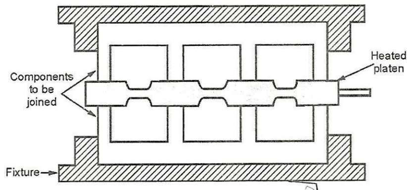
Figure 4.16 Hot-platen welding
