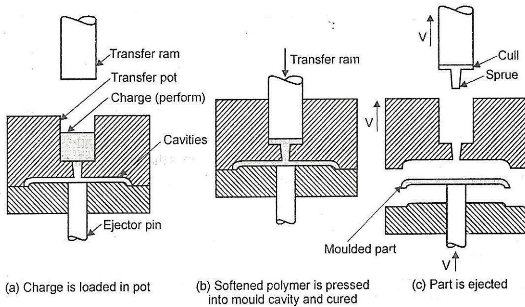
Figure 4.3 Transfer Moulding Advantages of Transfer Moulding
