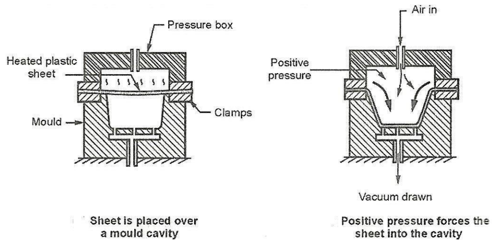
Figure 4.9 Pressure Thermoforming Advantages of thermoforming
