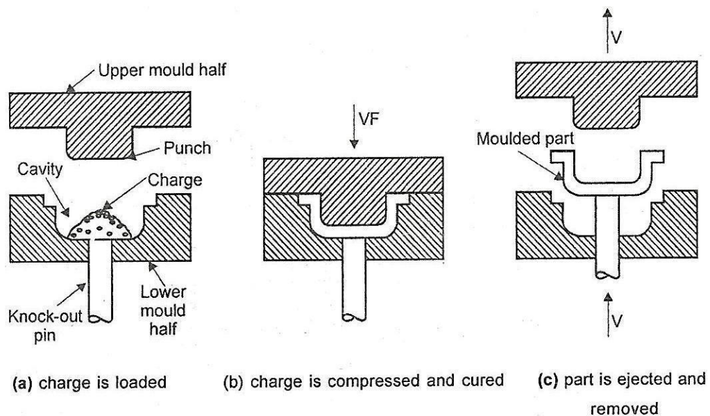
Figure 4.2 Compression Moulding
