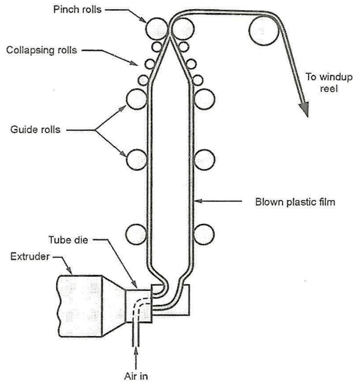
Figure 4.11 Extrusion of Film
