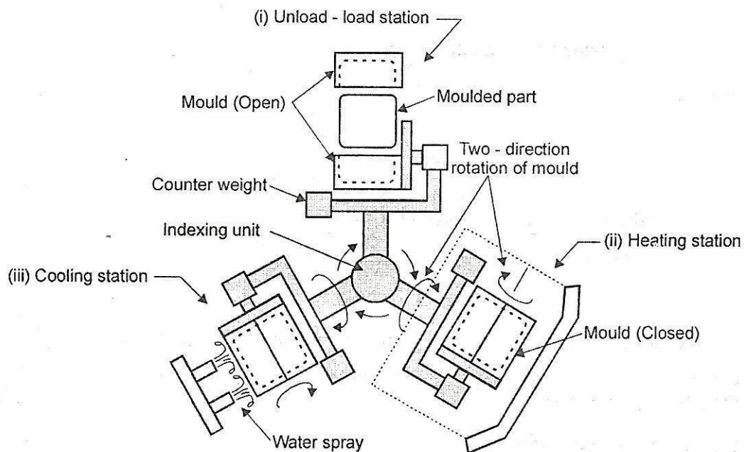
Figure 4.13 Rotational Moulding
