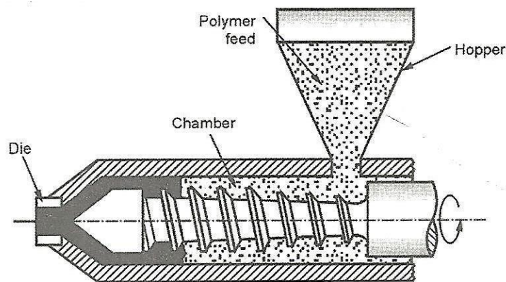
Figure 4.10.Extrusion
