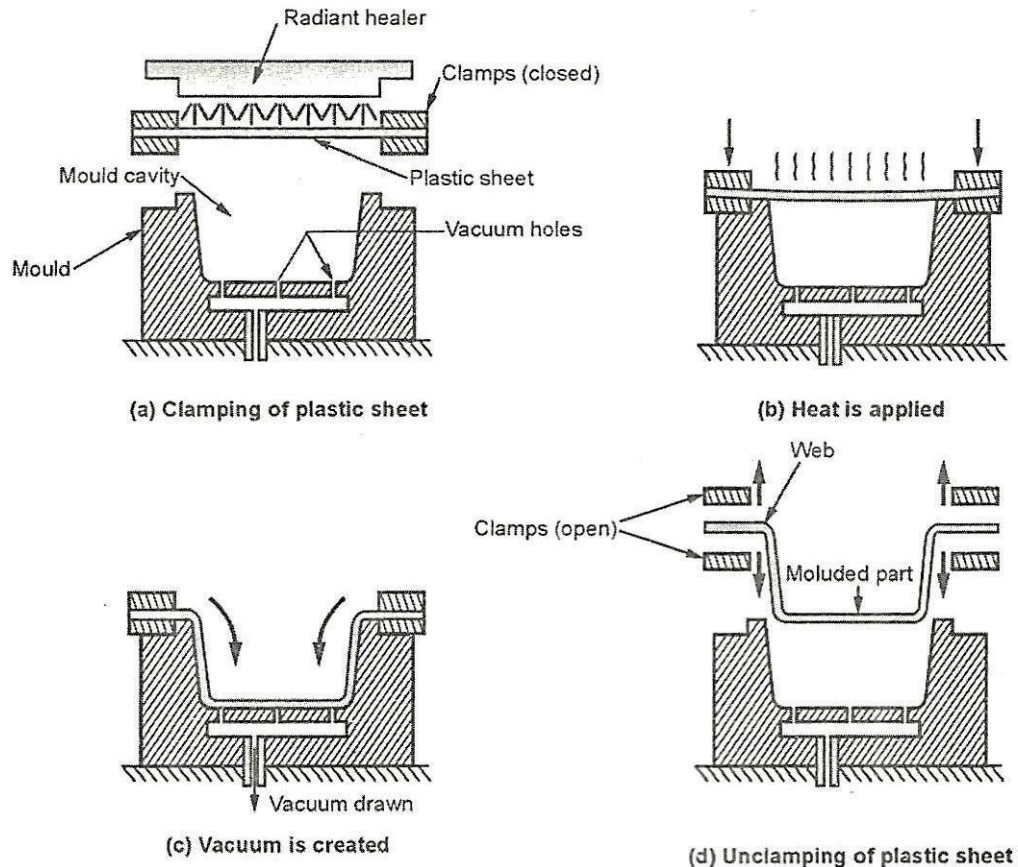
Figure 4.8 Vacuum forming
