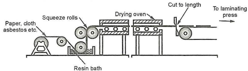
Figure 4.14. Laminating Processes
