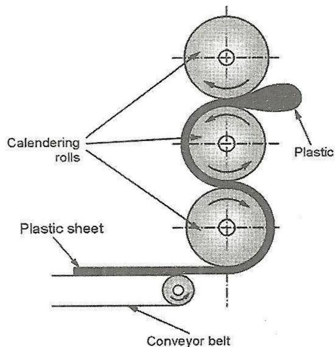
Figure 4.12. Calendering process
