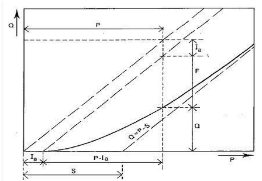
Fig. 12.1. Accumulated runoff Q versus accumulated rainfall P according to the Curve number Method. (Source: http://edepot.wur.nl/183157 )
