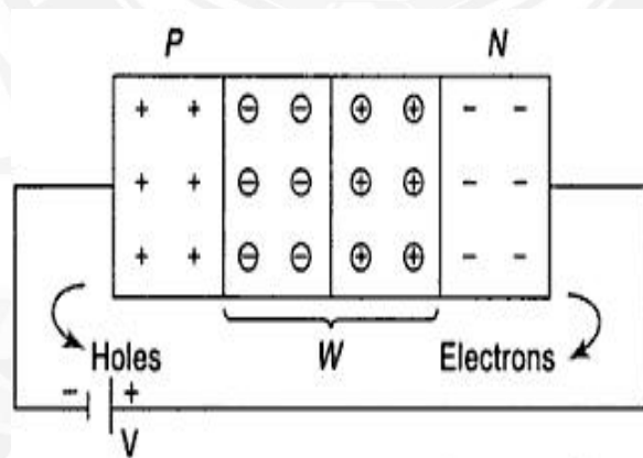
Figure: 1.1.3 PN junctions under reverse bias
