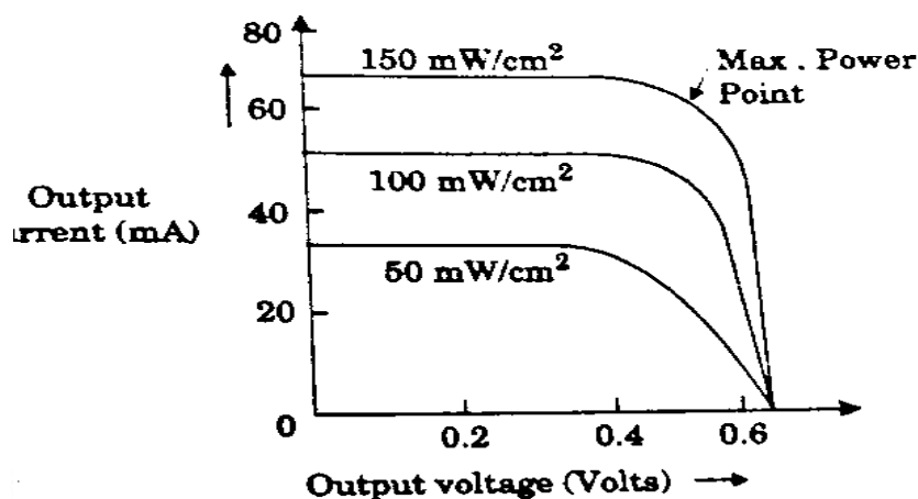
Fig 4.4.3 V-I characteristics
