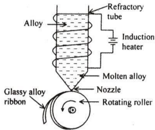
Figure.5.4- Melt spinning technique
