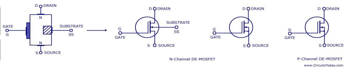
Schematic Symbols For a DE-MOSFET's
