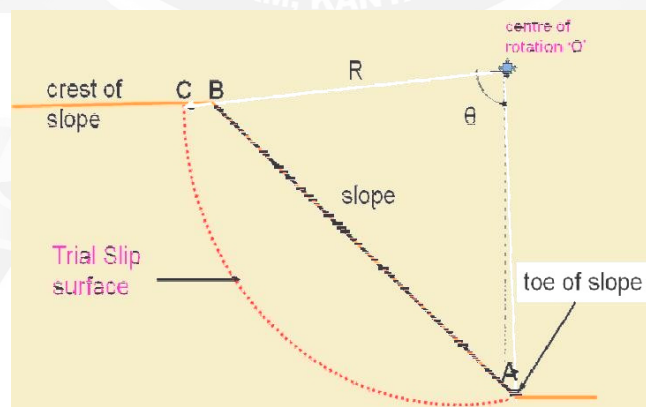
Fig 5.15 Trial circular slip surface (Arc AC)
