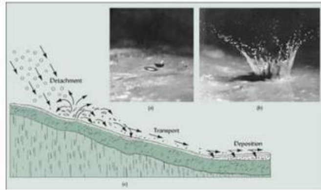
Fig. 2. Splash erosion.
