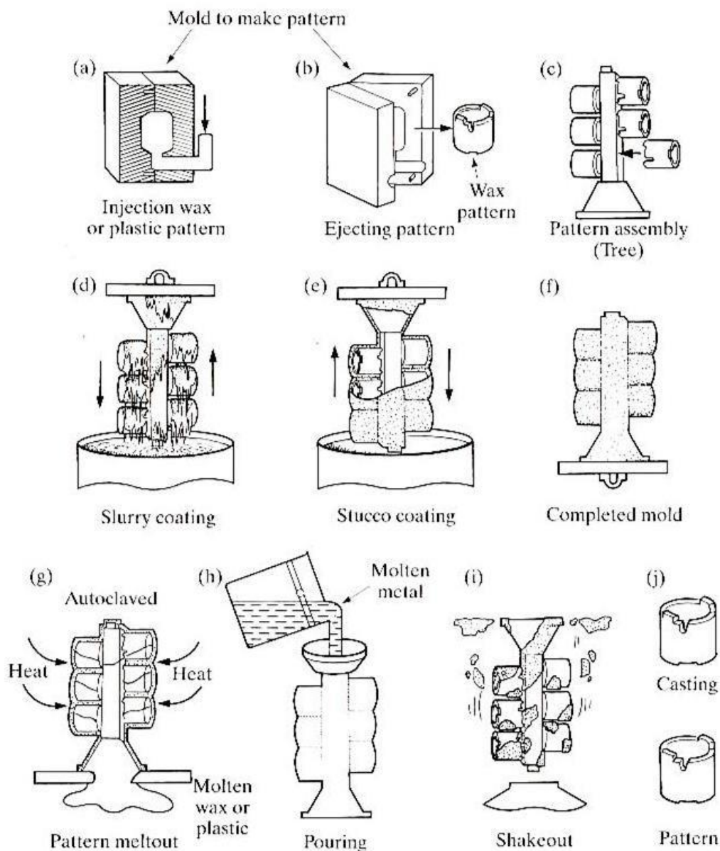
Figure 1.43 Investment Casting
