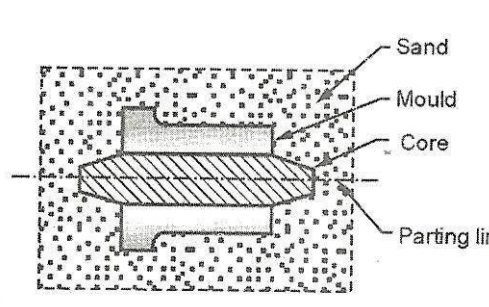
Figure 1.19 Horizontal Core
