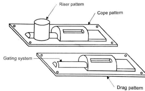
Figure: 1.7. Cope and drag pattern
