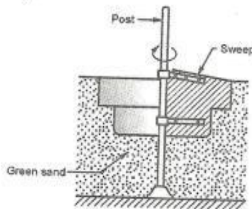
Figure: 1.10 Sweep pattern
