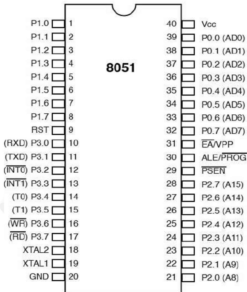
Figure 4.1.5 8051 Pin Configuration
