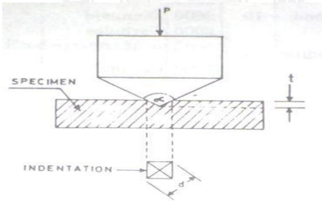
Square based pyramid indenter in Vicker's test
