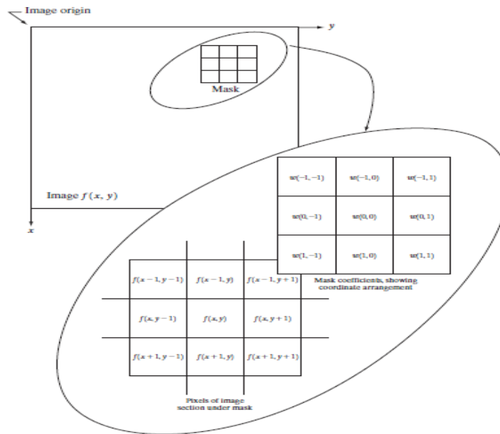
Figure 8 The mechanics of spatial filtering. The magnified drawing shows a 3*3 mask and the image section directly under it; the image section is shown displaced out from under the mask for ease of readability.
