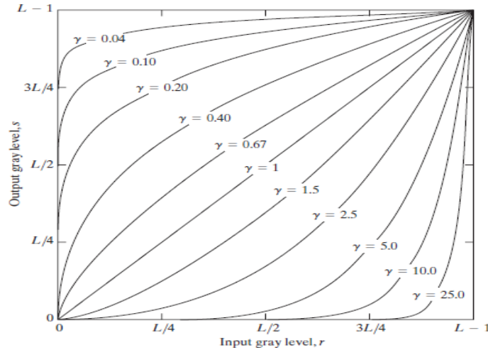
Figure 4: Plots of the equation s = c r^g for various values of g ( c=1 in all cases).
