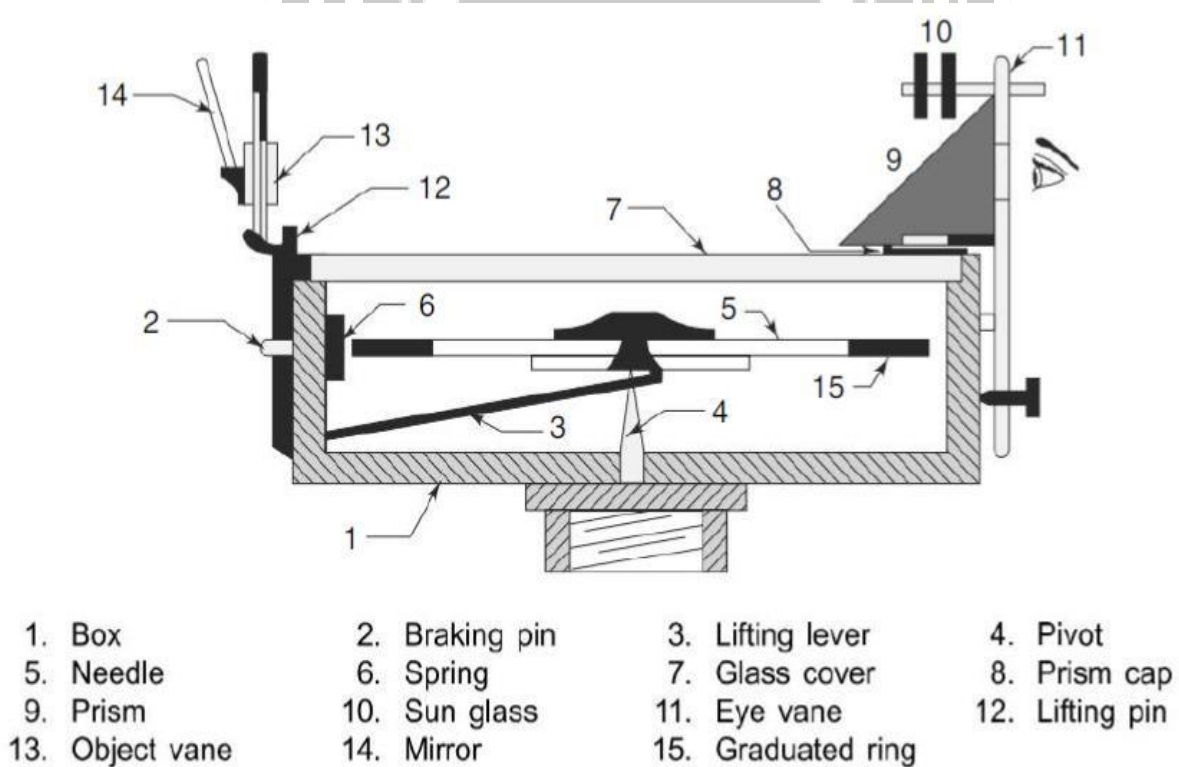
Prismatic Compass
