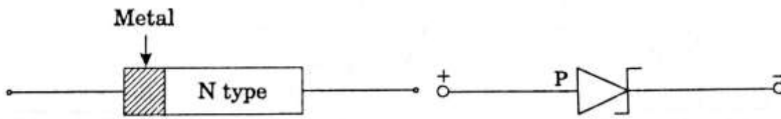
Fig 3.7..1 schottky diode and its circuit symbol
