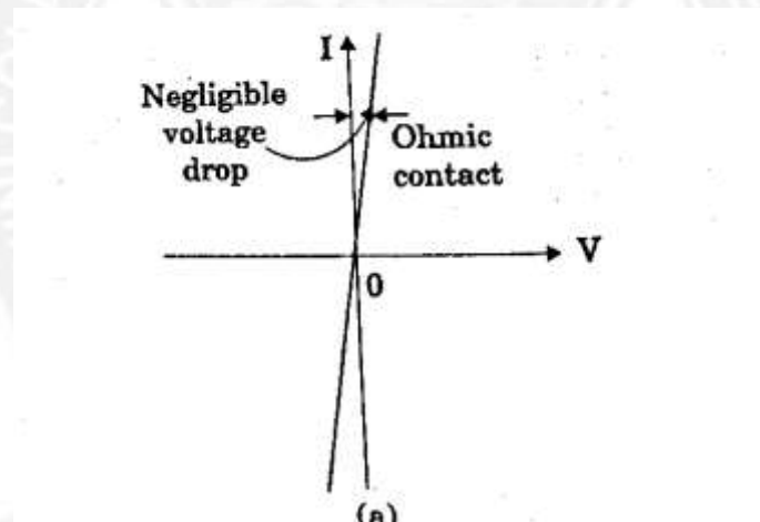
Fig 3.7.3;.V-I Characteristics
