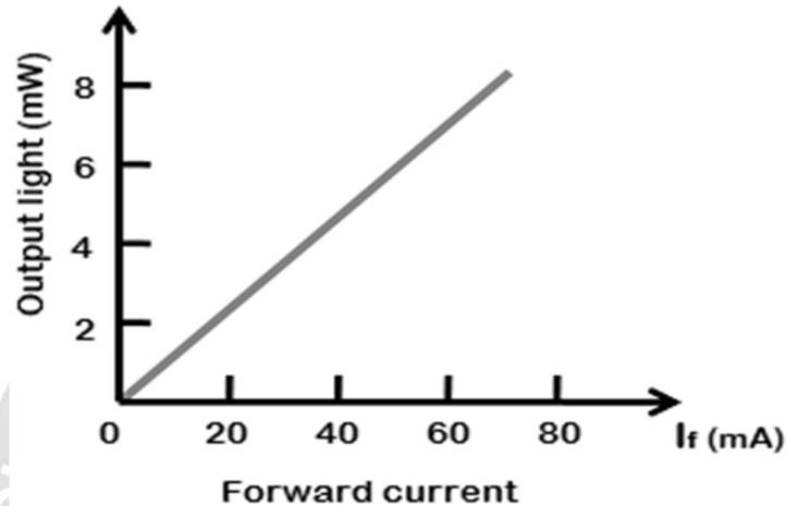
Fig:6 Characteristics of Light Emitting Diode
