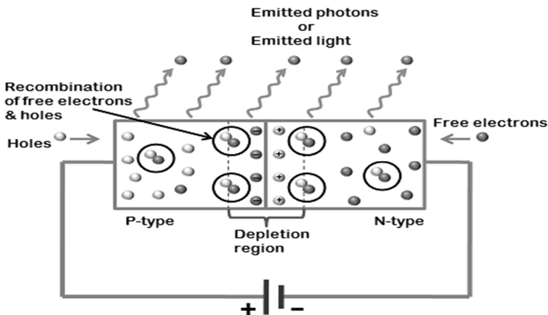
Fig:1 Working of Light Emitting Diode
