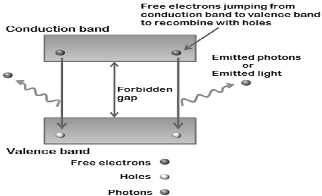
Fig:2 Process of Light Emission in LED
