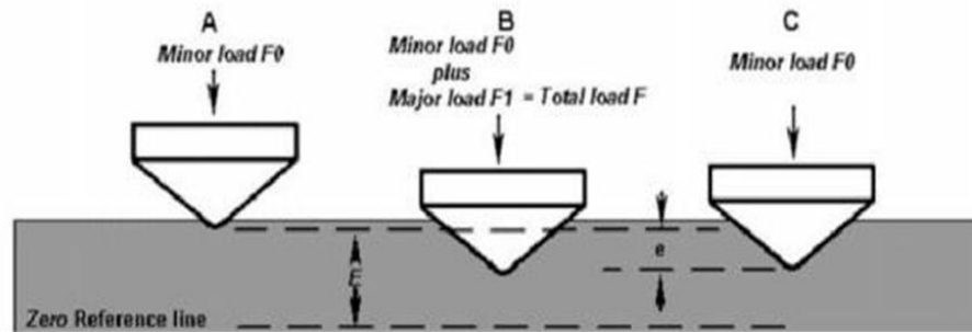
Fig. 1.Rockwell Principle
