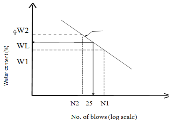
Fig 1.8 Flow Curve
