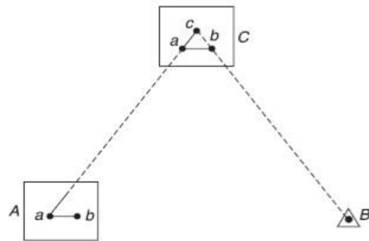
Resection by back ray
