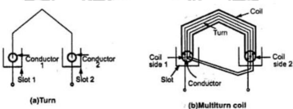
Figure 1.8 Single and Multicoil turn
