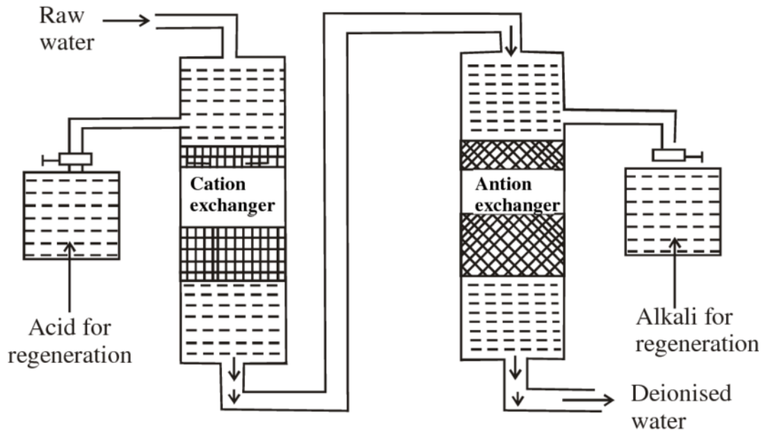
Figure 1.7.1 Demineralization process
