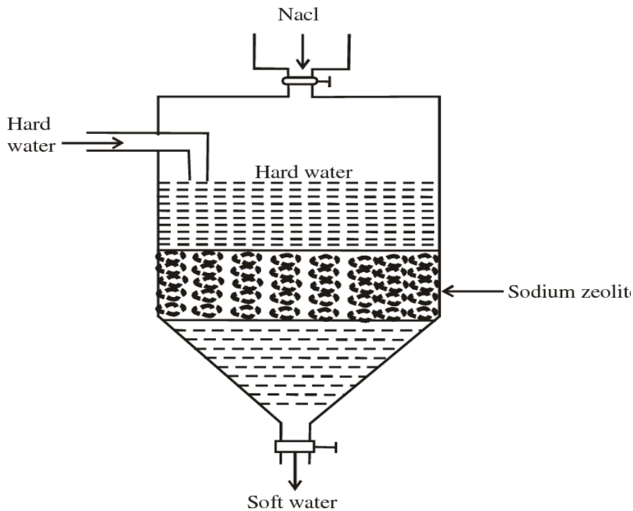
Figure.1.7.2 Zeolite process
