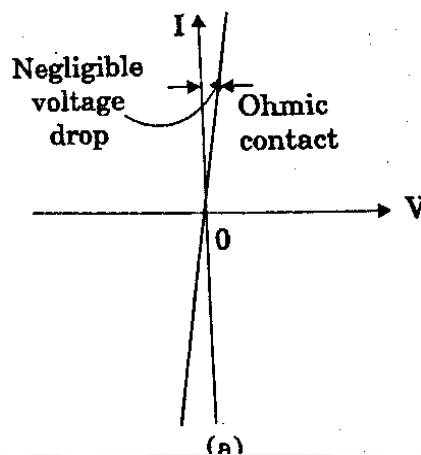
Fig 3.7.3;. V-I Characteristics
