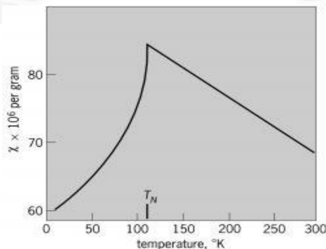
Fig 3.2.2. Variation of susceptibility with temperature
