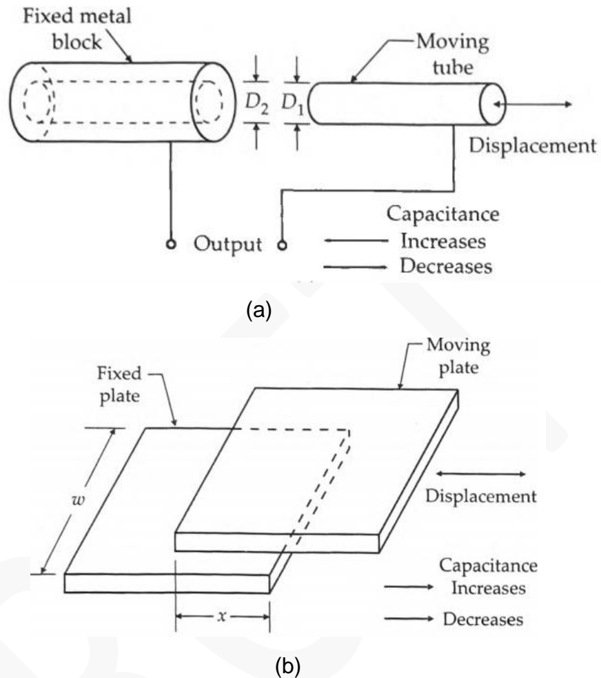
Figure.2 Capacitive transducers working on the principle of change of capacitance with change of area.
