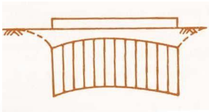
Fig 2: Contact Pressure Distribution - Flexible Footing - Cohesionless Soil
