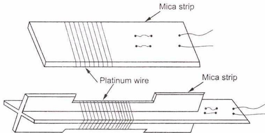
Fig 5.4.1 Resistance Thermometer
