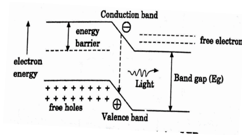
Fig 4.5.2. Energy band
