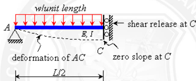
1.6.Reduced system AC is adopted for analysis for beam AB
