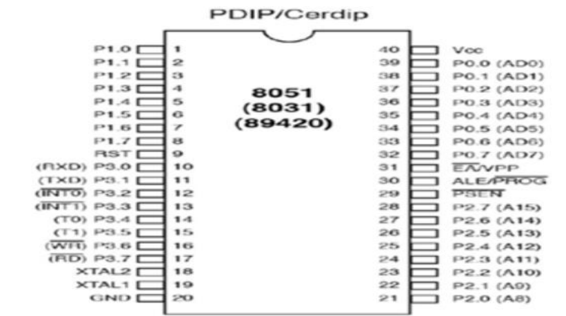
Figure 1.1 8051 microcontroller (40 pins IC)
