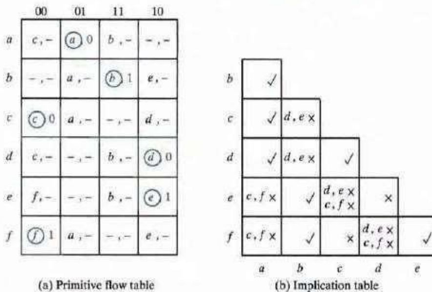
Fig 4.5.5 – a. Primitive Flow Table, b). Implication table
