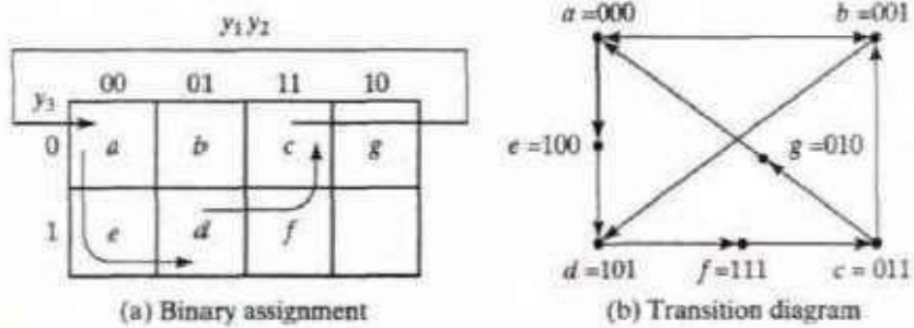
Fig 4.5.9 – a).Binary Assignment, b).Transition diagram
