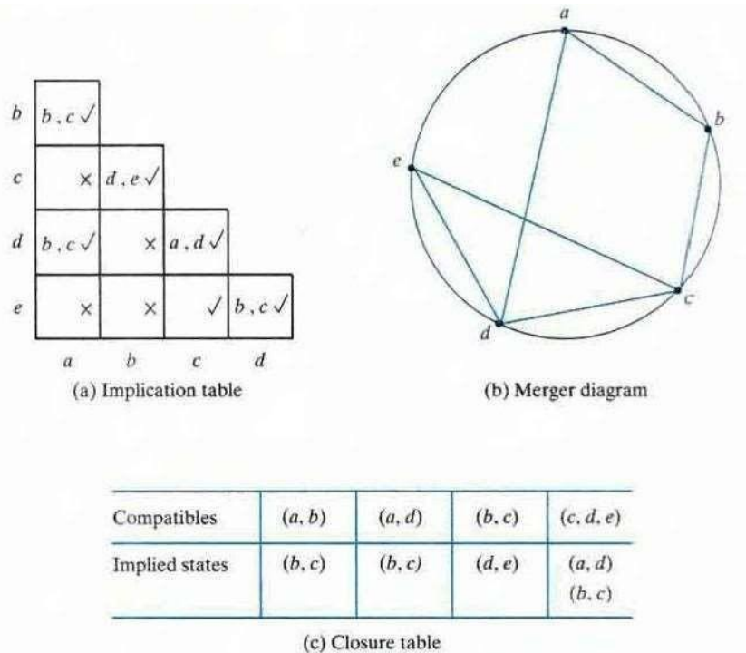
Fig 4.5.7 – a). Implication Table, b).Merger Diagram, c). Closure Table
