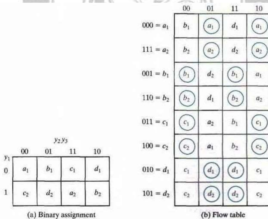
Fig 4.5.10 – a).Binary Assignment, b).Flow Table
