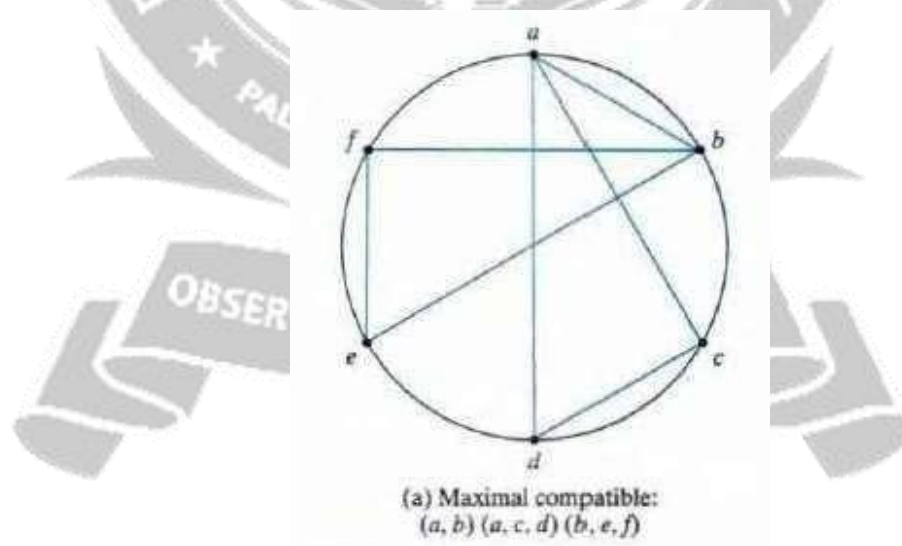
Fig 4.5.6 – Merger Diagram
