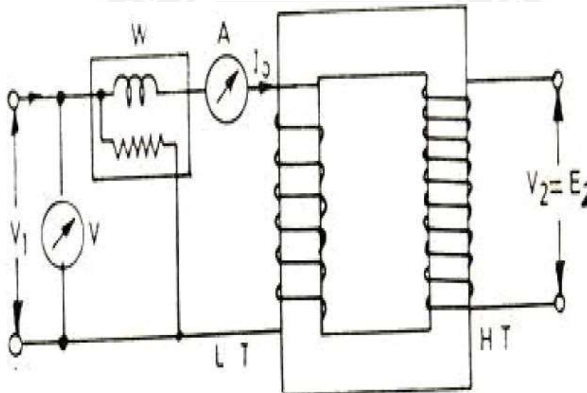
Figure. 4.3.1 Open Circuit
