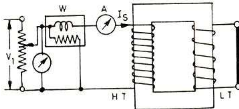
Figure 4.3.2 Short Circuit
