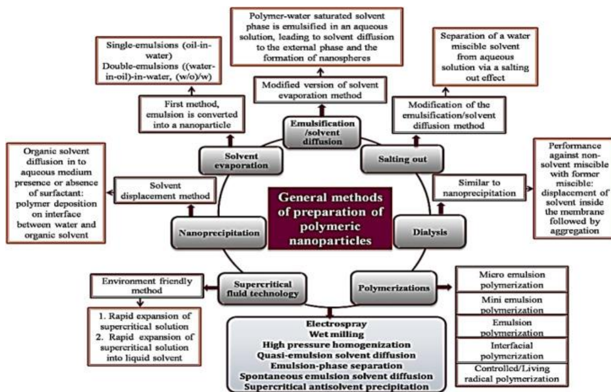
Schematic showing various techniques for the preparation of PNPs
